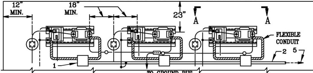
ARRANGEMENT OF EQUIPMENT WHEN OUTDOOR TYPE INSTRUMENT TRANSFORMERS ARE INSTALLED
